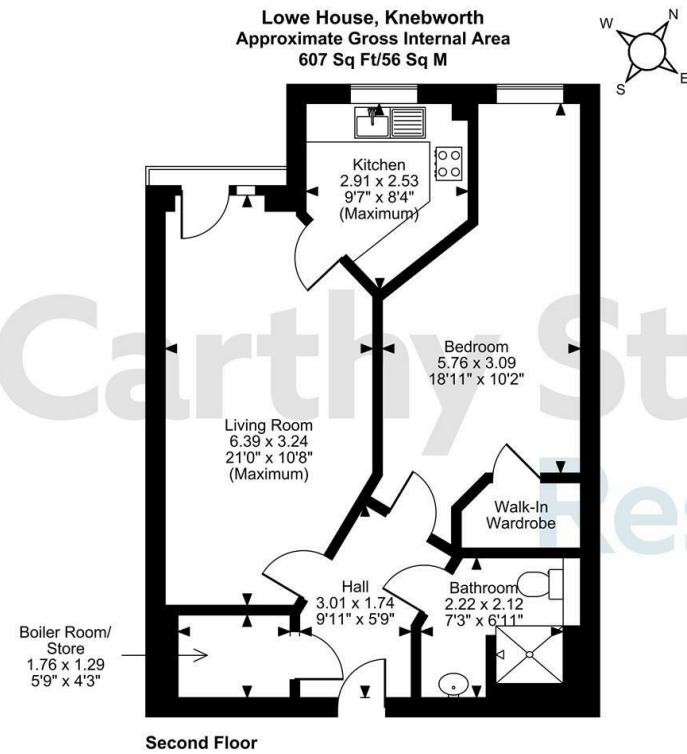
Second Floor FOR ILLUSTRATIVE PURPOSES ONLY - NOT TO SCALE The position & size of doors, windows, appliances and other features are approximate only. © ehouse. Unauthorised reproduction prohibited. Drawing ref. dig/8635811/CGI
