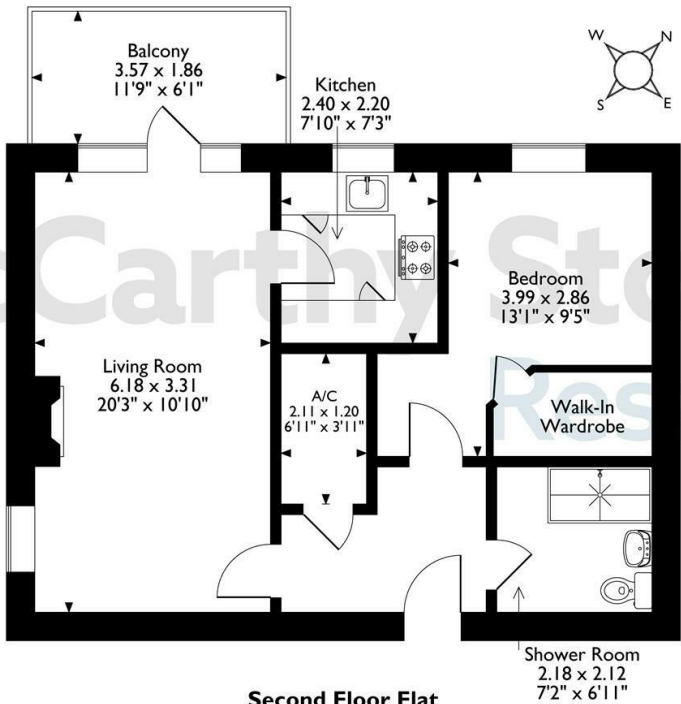
Second Floor Flat The position & size of doors, windows, appliances and other features are approximate only. © ehouse. Unauthorised reproduction prohibited. Drawing ref. dig/8659547/DST.
