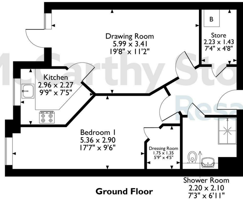
The position & size of doors, windows, appliances and other features are approximate only. © ehouse. Unauthorised reproduction prohibited. Drawing ref. dig/8688739/DST.
