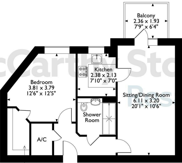
First Floor The position & size of doors, windows, appliances and other features are approximate only. © ehouse. Unauthorised reproduction prohibited. Drawing ref. dig/8681560/DST.
