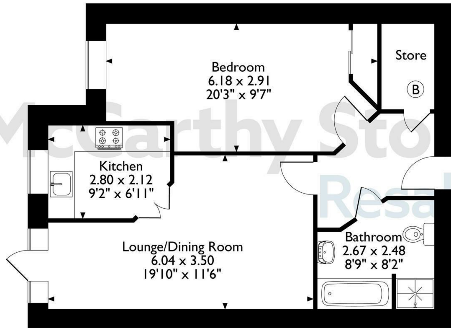
The position & size of doors, windows, appliances and other features are approximate only. © ehouse. Unauthorised reproduction prohibited. Drawing ref. dig/8692787/DST.
