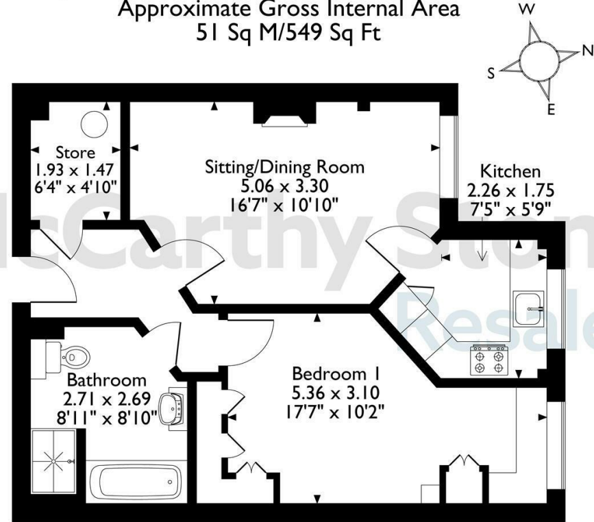
The position & size of doors, windows, appliances and other features are approximate only. © ehouse. Unauthorised reproduction prohibited. Drawing ref. dig/8695753/DST.
