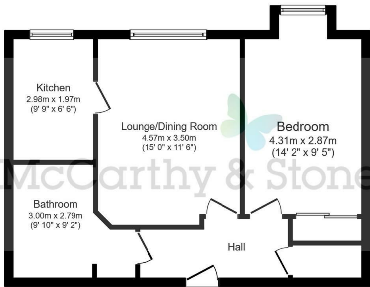
Floor Plan
