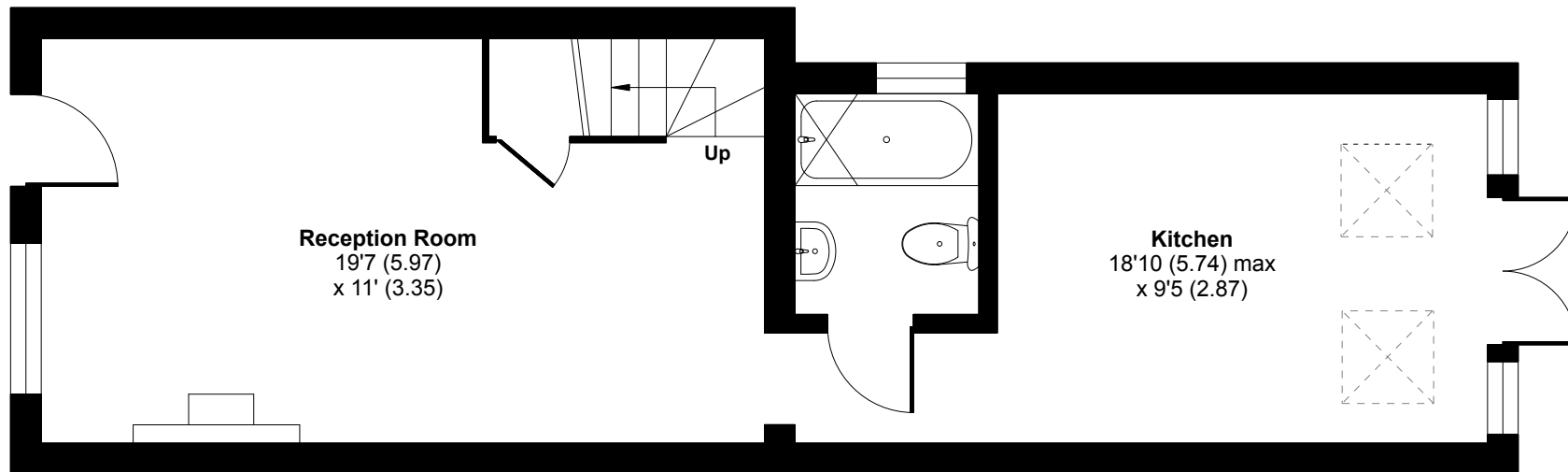
GROUND FLOOR
