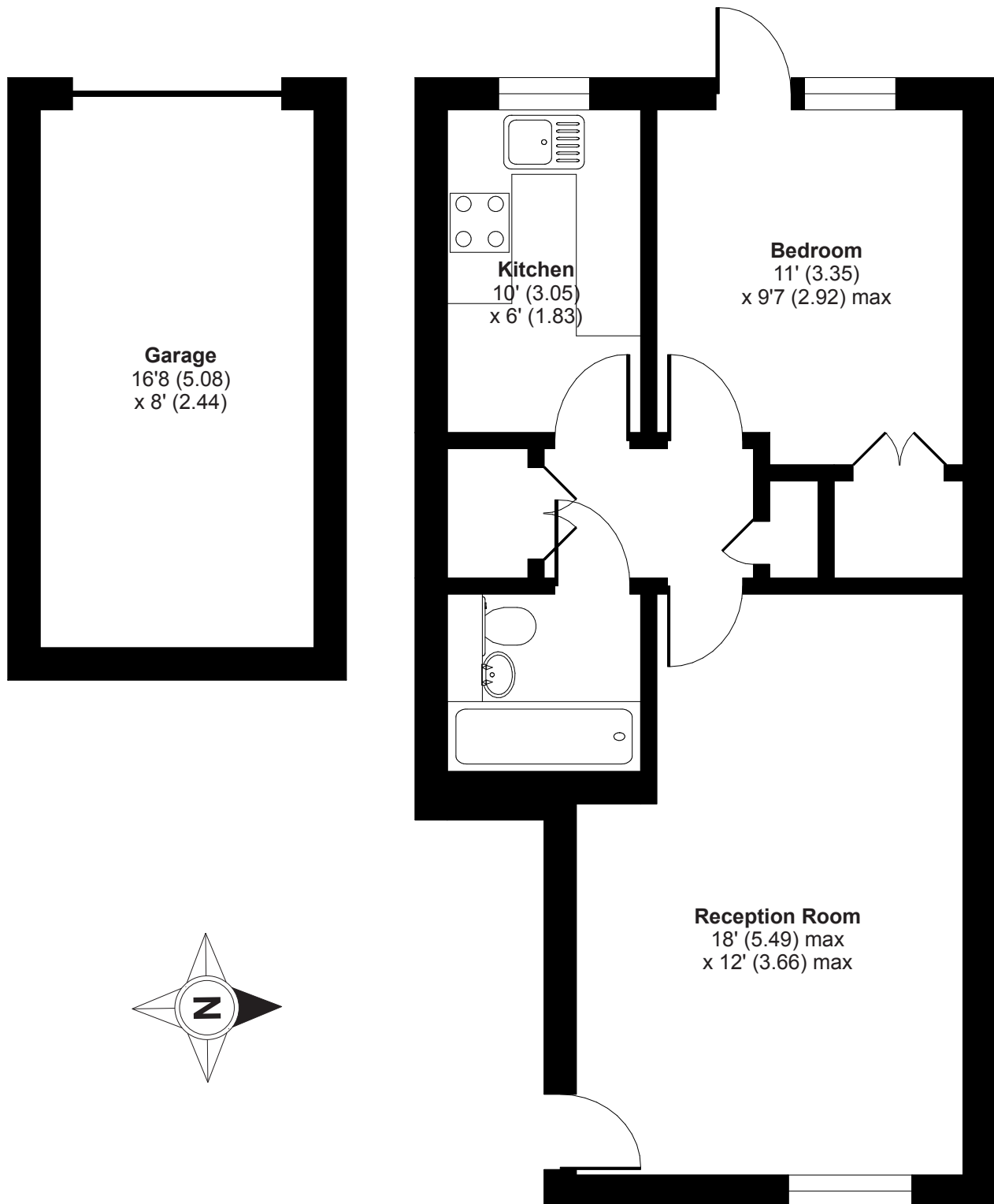
GROUND FLOOR
