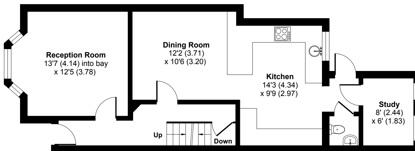
GROUND FLOOR
