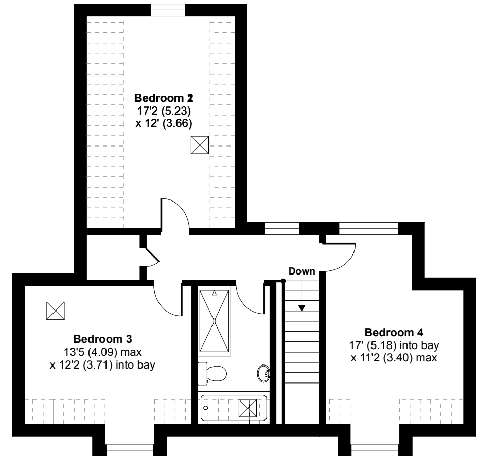
FIRST FLOOR
