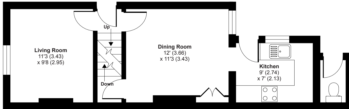
GROUND FLOOR
