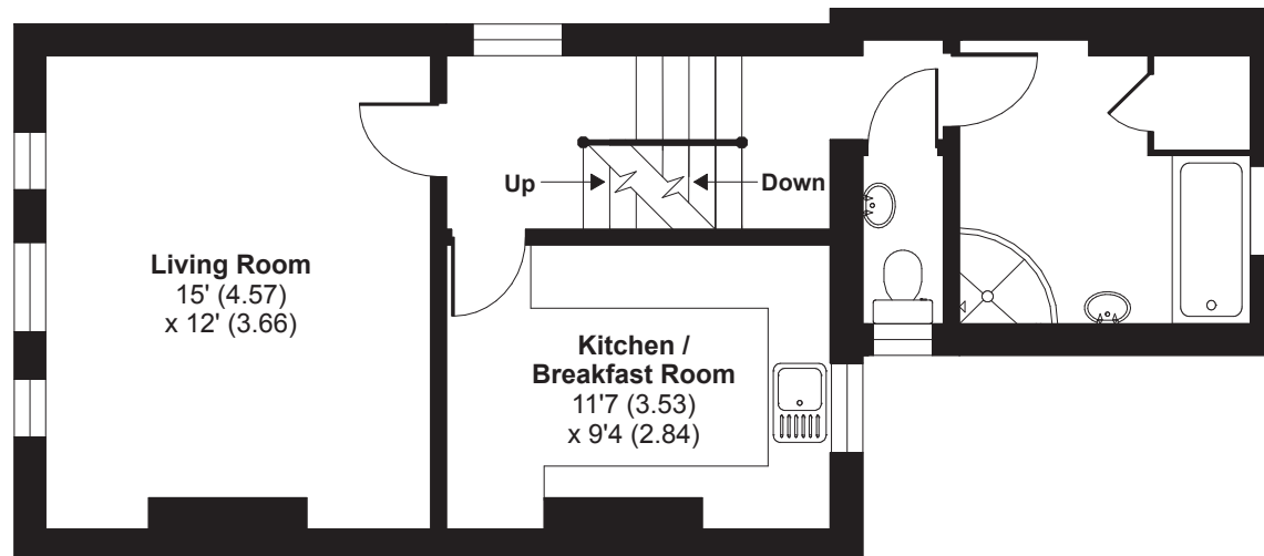
FIRST FLOOR
