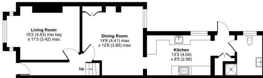
GROUND FLOOR
