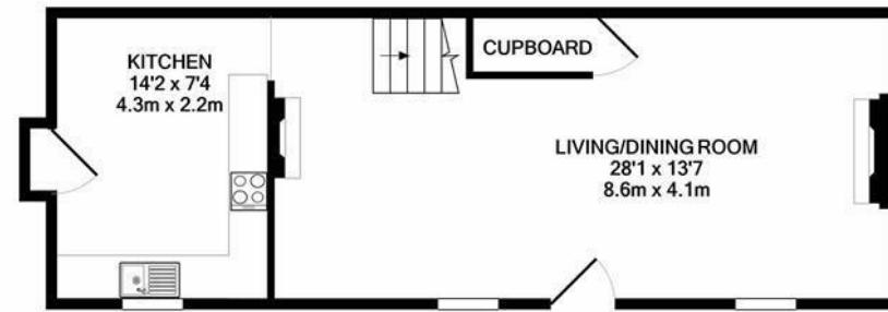
GROUND FLOOR
