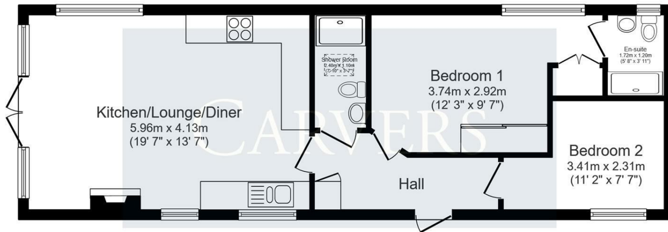
Ground Floor
