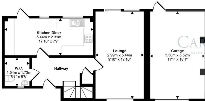
Ground Floor Approx 62 sq m / 672 sq ft
