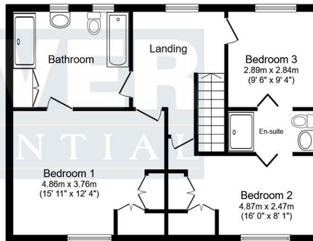
First Floor Floor area 61.4 sq.m. (660 sq.ft.)
