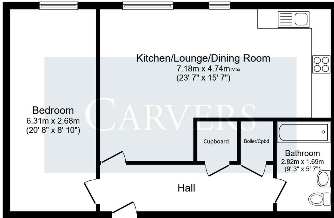
Floor Plan
