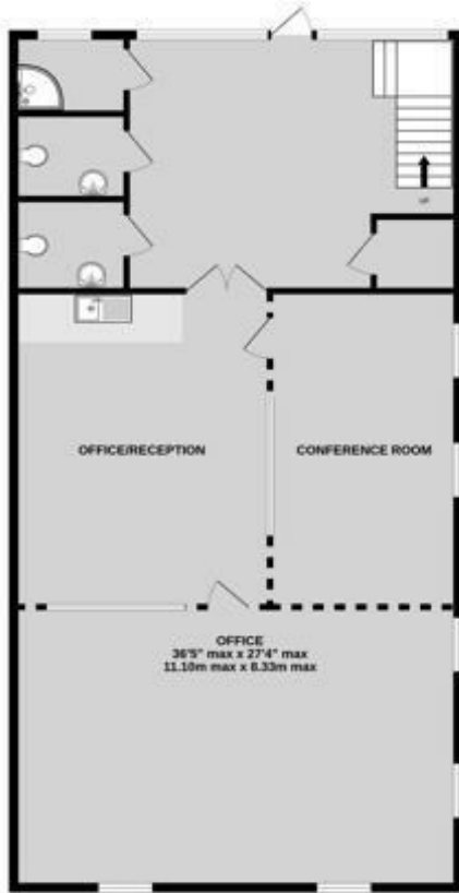
GROUND FLOOR 1419 sq.ft. (131.4 sq.m.) approx.
