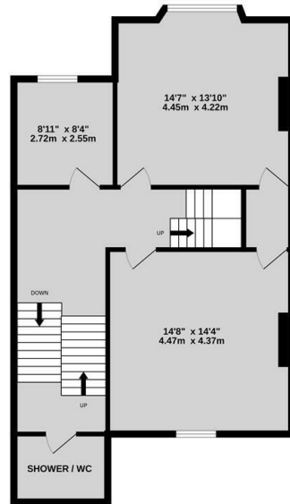
1ST FLOOR 788 sq.ft. (72.9 sq.m.) approx.
