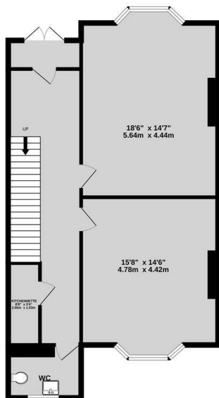
GROUND FLOOR 795 sq.ft. (73.0 sq.m.) approx.
