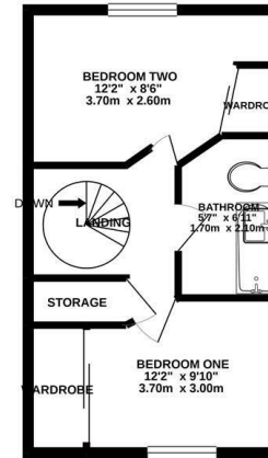
1ST FLOOR 312 sq.ft. (29.0 sq.m.) approx.
