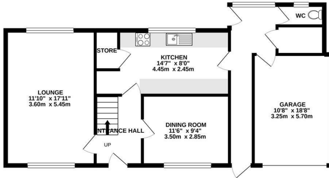
GROUND FLOOR 810 sq.ft. (75.2 sq.m.) approx.
