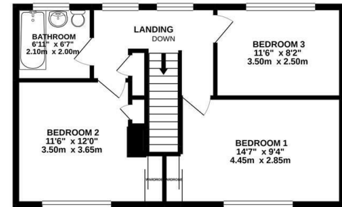
1ST FLOOR 523 sq.ft. (48.6 sq.m.) approx.
