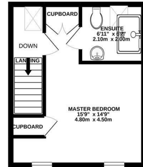
2ND FLOOR 262 sq.ft. (24.3 sq.m.) approx.
