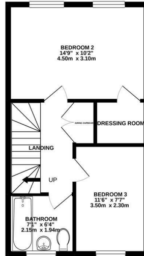
1ST FLOOR 392 sq.ft. (36.4 sq.m.) approx.
