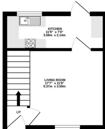
GROUND FLOOR 194 sq.ft. (18.0 sq.m.) approx.
