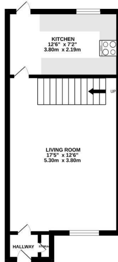
GROUND FLOOR 321 sq.ft. (29.8 sq.m.) approx.
