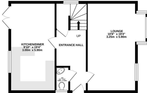
GROUND FLOOR 543 sq.ft. (50.4 sq.m.) approx.
