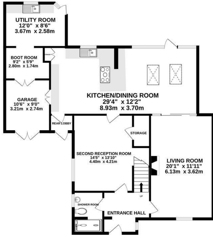
GROUND FLOOR 1400 sq.ft. (130.0 sq.m.) approx.
