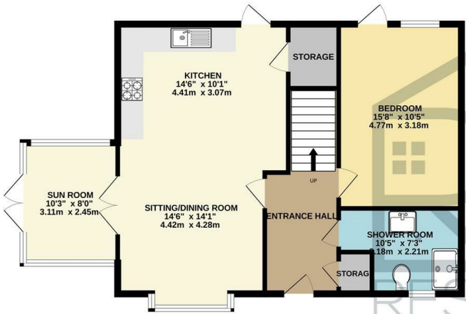
GROUND FLOOR 720 sq.ft. (66.9 sq.m.) approx.
